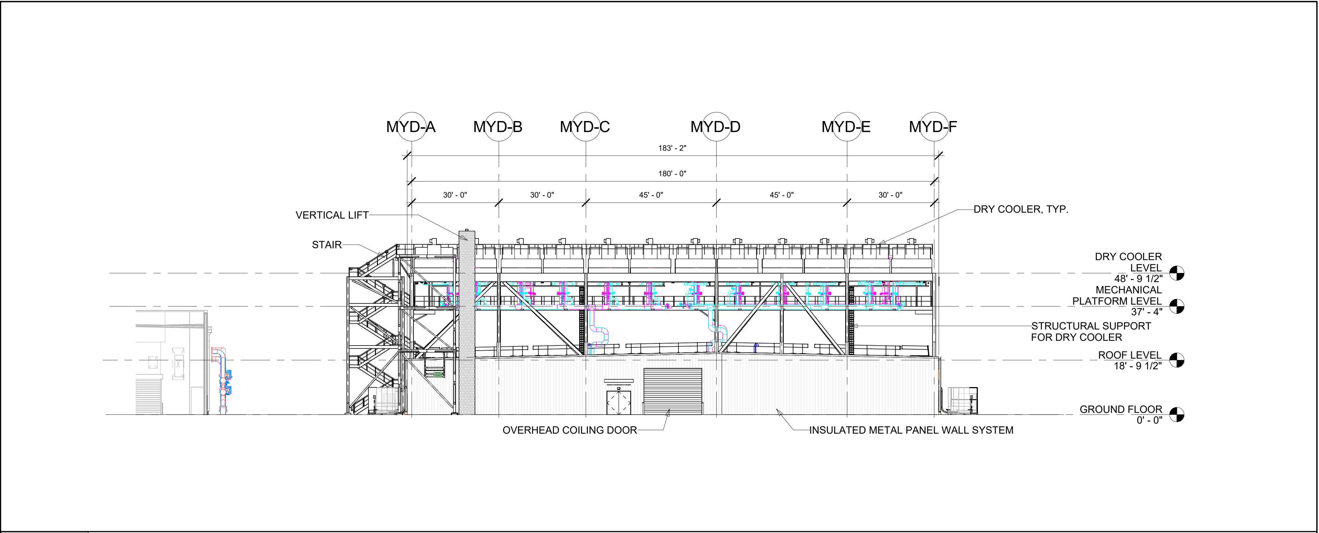
4 BUILDING ELEVATION - SIDE 2
