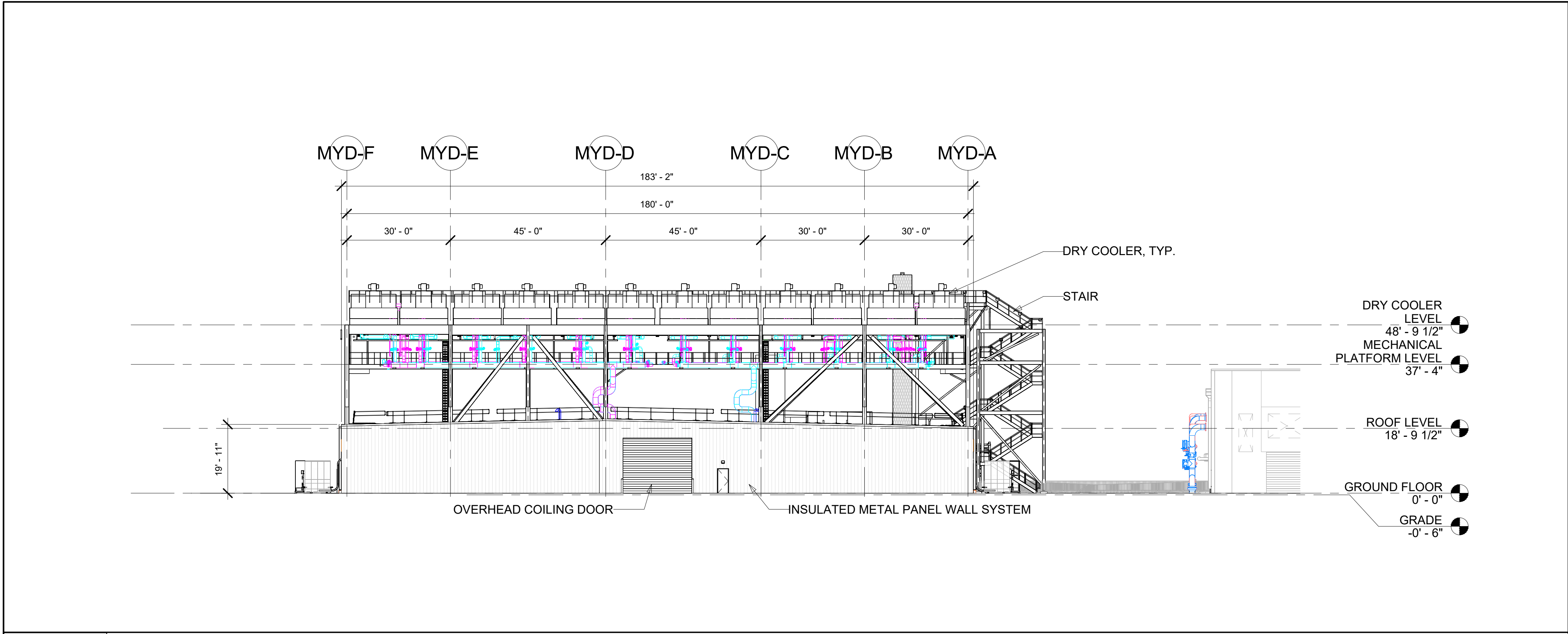
3 BUILDING ELEVATION - SIDE 1
